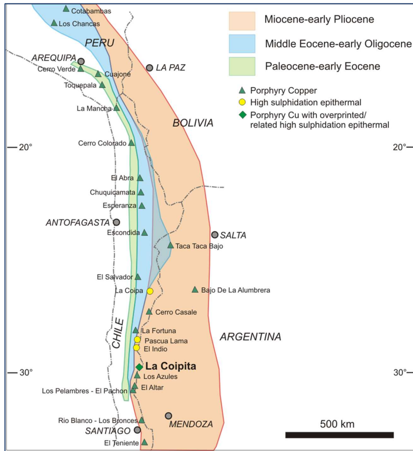
Figure 2 – Geological Setting
